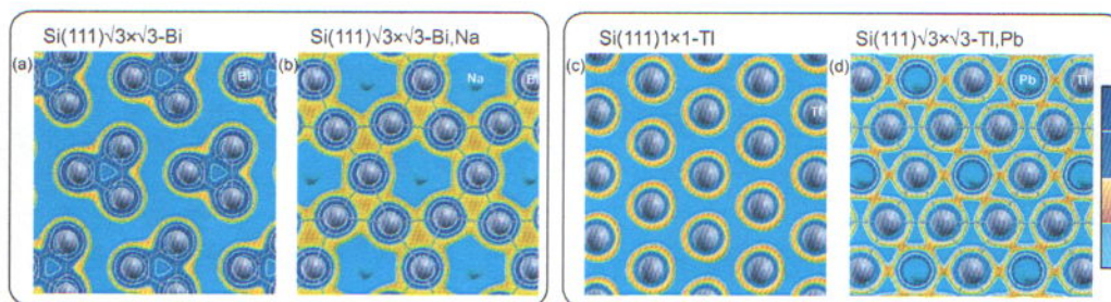
Figure 4 | Calculated electron density maps for (a) Bi/Si(111) \sqrt{3} \times \sqrt{3} , (b) (Bi, Na)/Si(111) \sqrt{3} \times \sqrt{3} , (c) Tl/Si(111) 1 \times 1 , and (d) (Tl, Pb)/Si(111) \sqrt{3} \times \sqrt{3} surfaces. The multi-colour (blue-yellow) scale for electron density is used to highlight the interconnected electron density network at metallic alloy surfaces.
